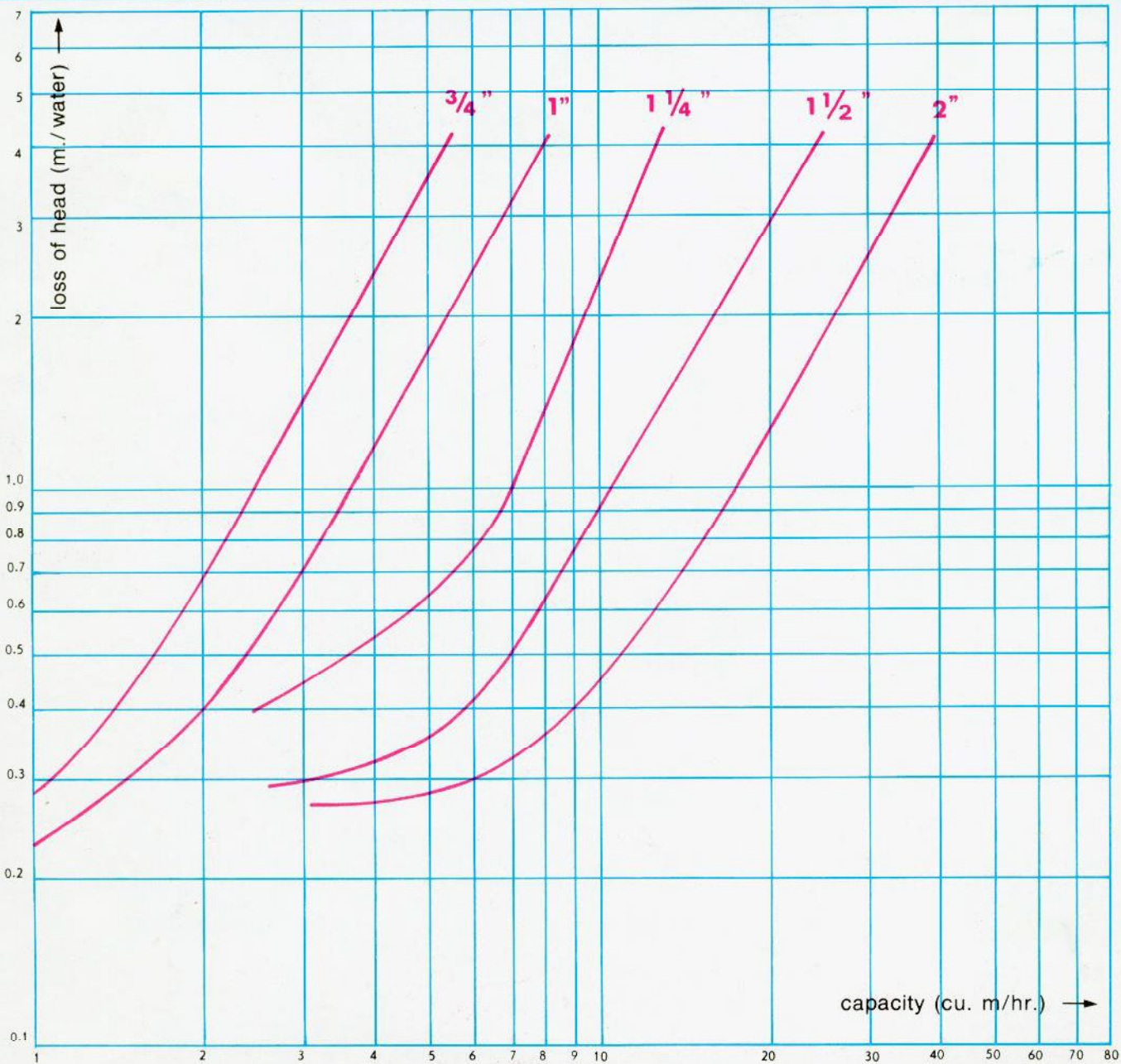
GRAPH OF LOSS OF HEAD RELATIVE TO CAPACITY
